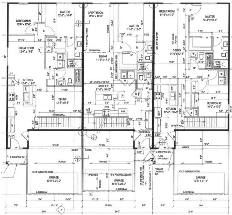
UNIT 'A' = 1136 SQ. FT. UNIT 'B' = 1044 SQ. FT. UNIT 'C' = 1136 SQ. FT. MAIN FLOOR PLANS
